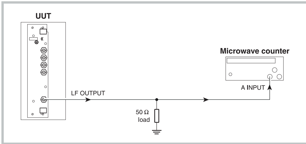
Fig. 5-11 Modulation oscillator frequency test set-up
